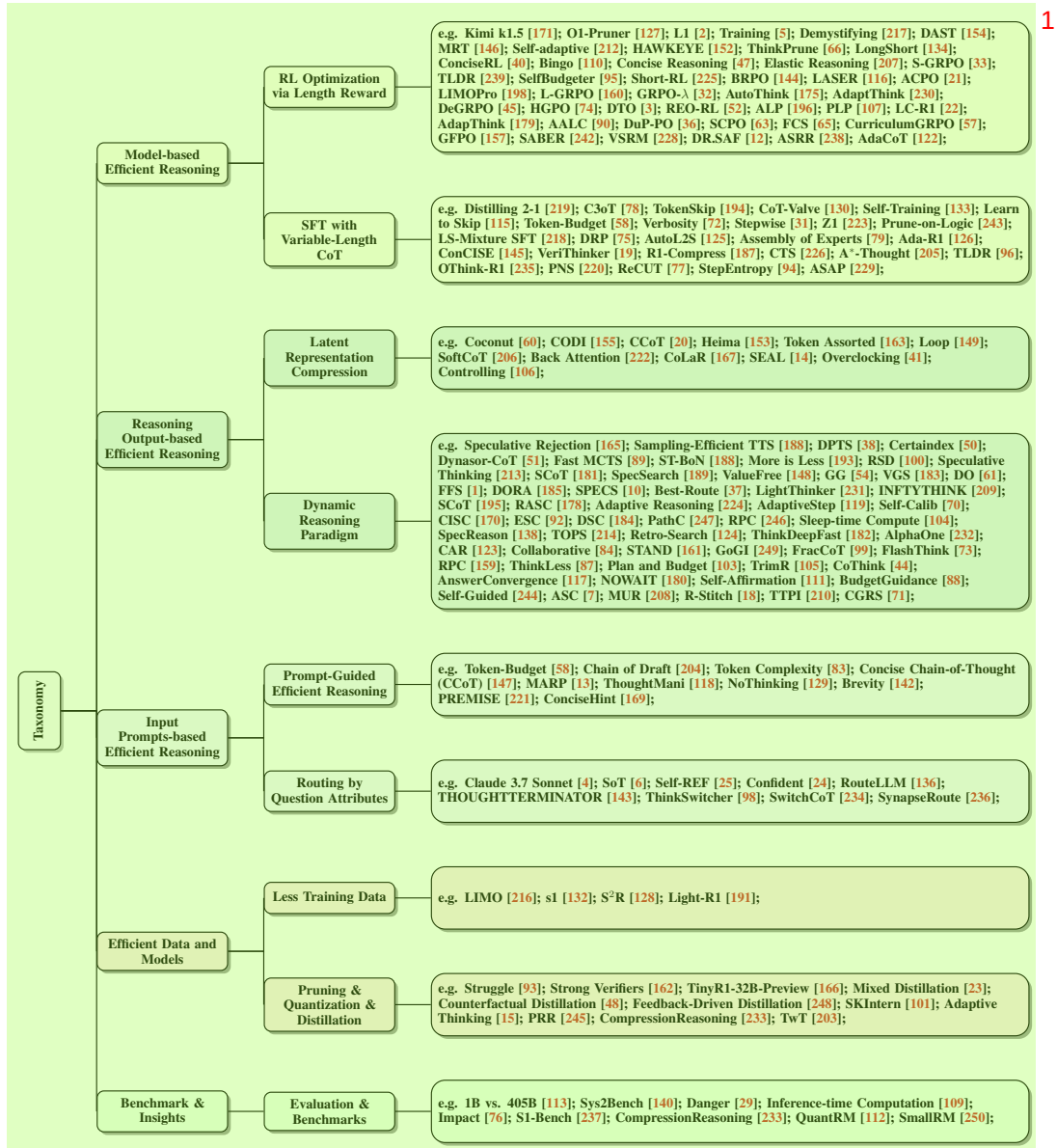
Figure 3: Taxonomy of existing literature on efficient reasoning for LLMs. 2
