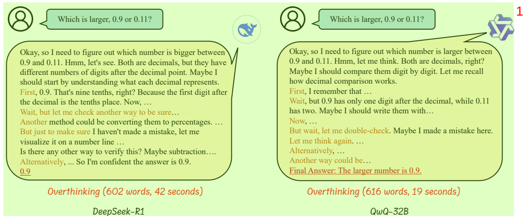
Figure 4: An example of the “overthinking phenomenon”: when asked “Which is larger, 0.9 or 0.11?”, the reasoning model takes an unnecessarily long time (e.g., 19 seconds for QwQ-32B [172] and 42 seconds for DeepSeek-R1 [56]) to arrive at the correct answer. This example was tested in March 2025.
