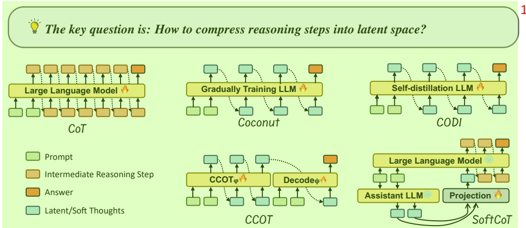
Figure 7: Comparison of methods of compressing reasoning steps into fewer latent representations.2
